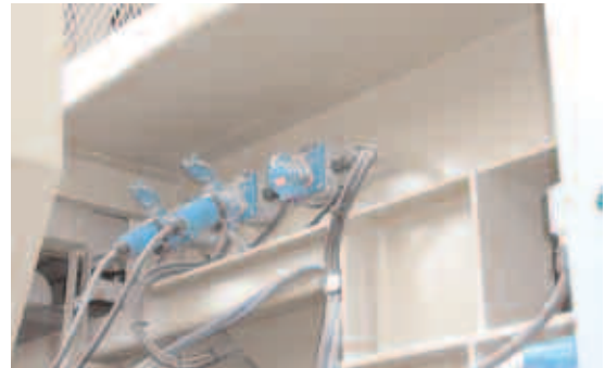
Closeup shows multiple connections that facilitate ease of moving portable plant components.
