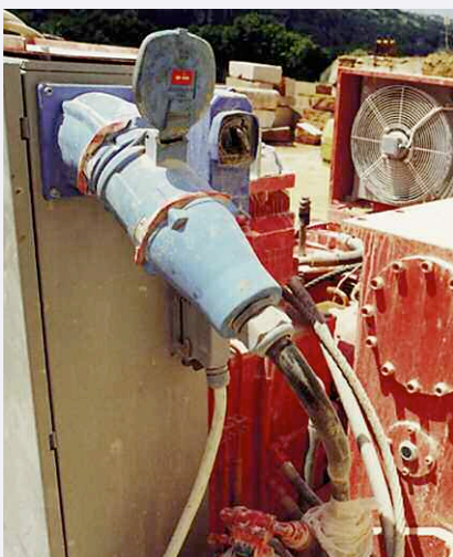
Power connections to a marble cutter
