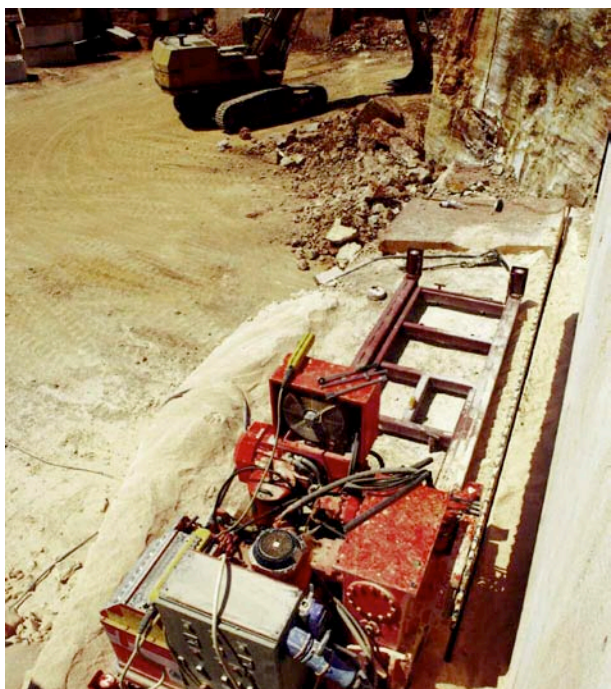
Meltric DS devices supply power to large cutting machines at a marble quarry. DS's are UL and CSA switch rated, allowing them to function as a 'line of sight' disconnect.
